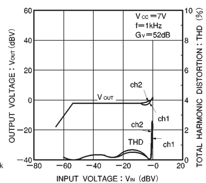
Fig. 17 ALC characteristics
