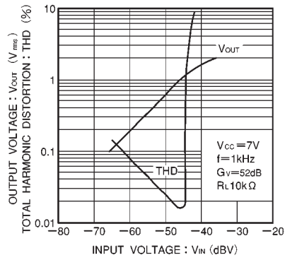
Fig. 18 Input/output characteristics
