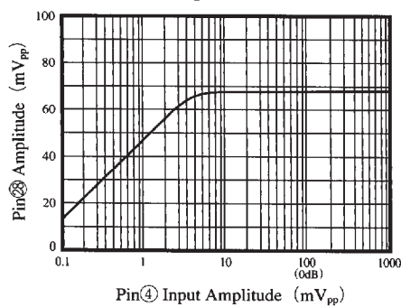
Limiter-Up Characteristics
