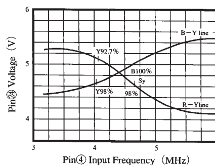
Discriminator S-Characteristics
