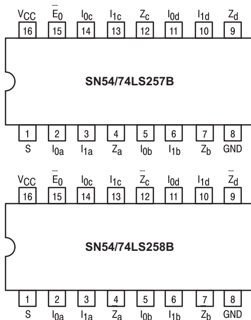
CONNECTION DIAGRAM DIP (TOP VIEW)
