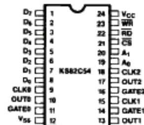
Figure 1b: 24-Pin Configuration
