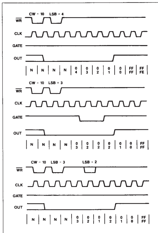
Figure 8: Mode 0 Timing
