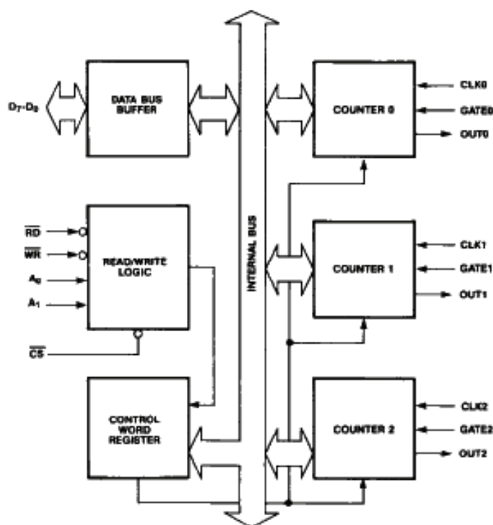
Figure 2: KS82C54 Block Diagram
