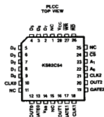
Figure 1a: Plastic Leaded Chip Carrier
