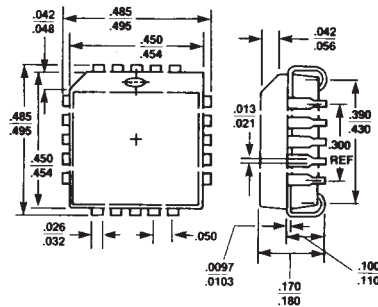
Figure 16: PLCC Package
