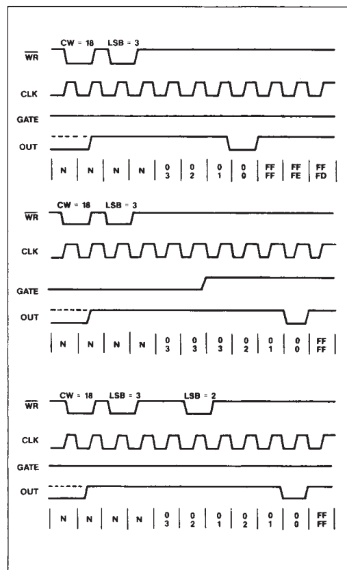
Figure 13: Mode 5 Timing
