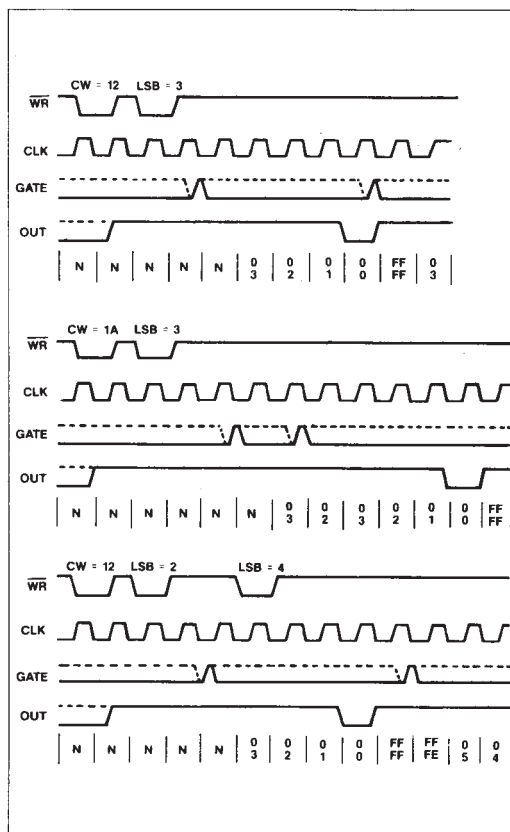
Figure 12: Mode 4 Timing
