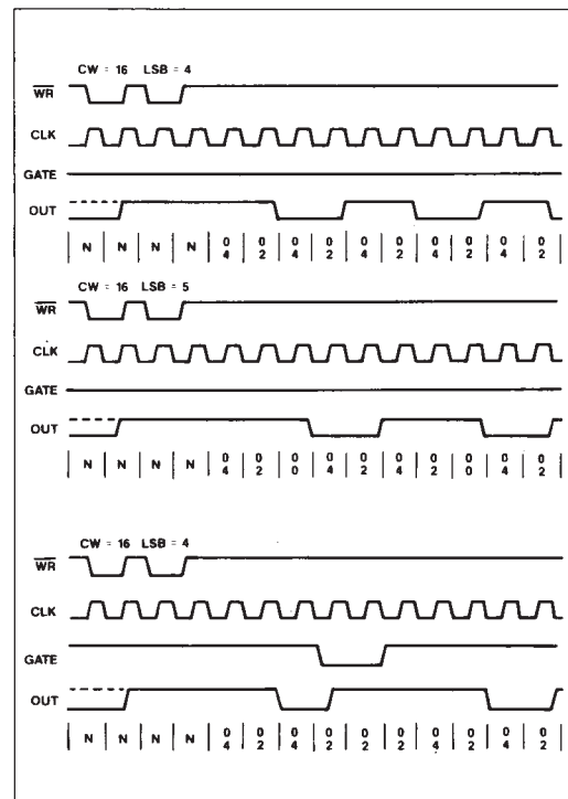
Figure 11: Mode 3 Timing
